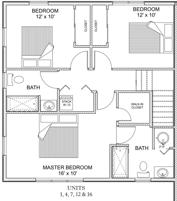
2 nd Floor
