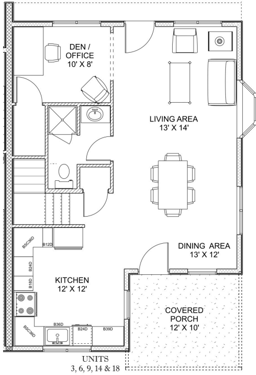
1 st Floor
