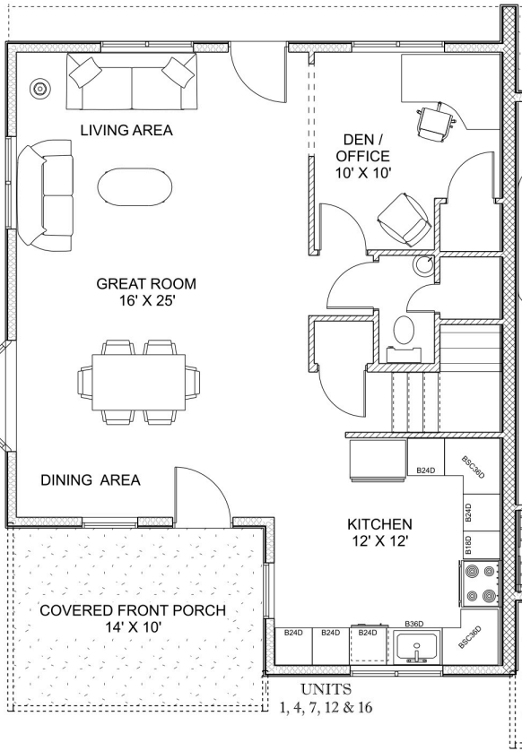
1 st Floor
