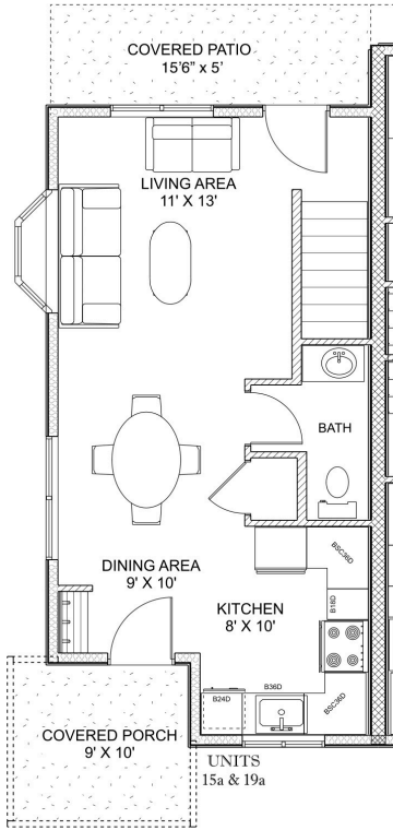
1 st Floor
